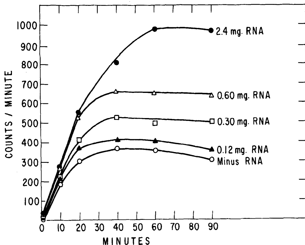
Fig. 1 - Dependence of C^{14} -L-valine incorporation into protein upon ribosomal RNA. The reaction mixture is presented in Table 1. Each reaction mixture contained 0.98 mg of E. coli soluble RNA (saturating concentration) and 4.4 mg of Incubated-S-30 protein.
